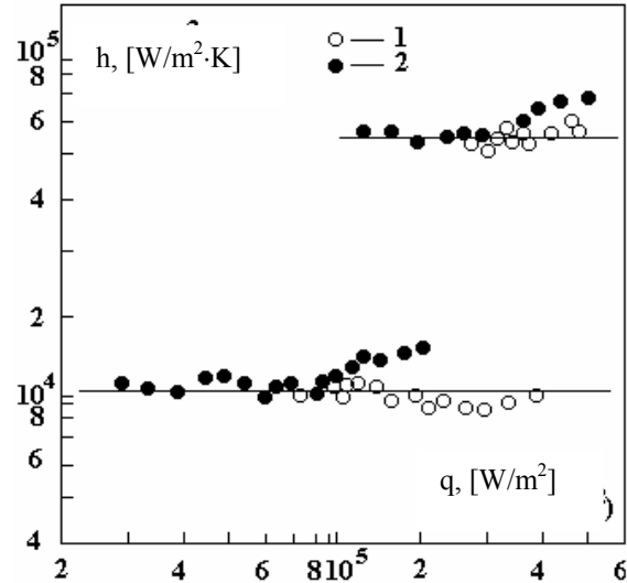
Figure 4. Comparison of equation (1) (horizontal lines) with experimental data [16] on steam condensation and distilled water evaporation on surfaces with triangular grooves ( \varepsilon = 0.5 mm) made of stainless steel (lower data) and cooper (upper data): 1 – condensation; 2 – evaporation
