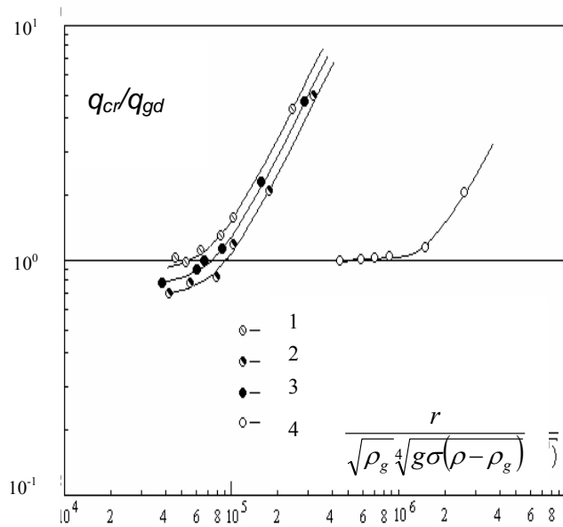
Figure 15. Experimental data [28] on CHF during pool boiling of dautherm-A (1), chlorbenzene (2), toluene (3), and water (4) at reduced saturation pressures; horizontal line - according hydrodynamic theory of Kutateladze [48]
