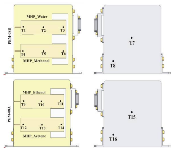
Figure 5: Thermocouples position.
