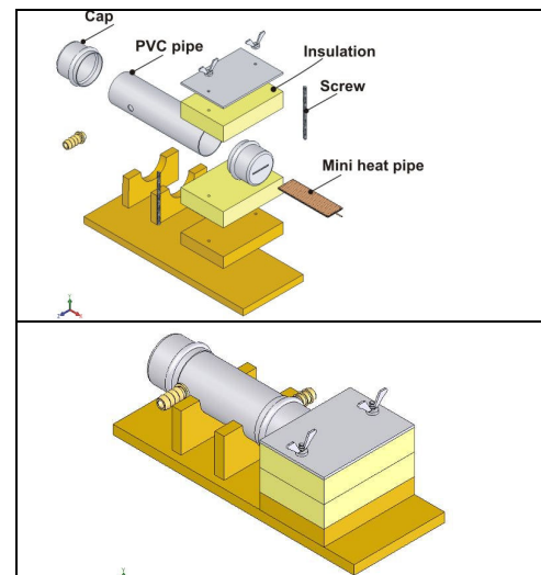
Figure 1: Experimental facility sketch.
